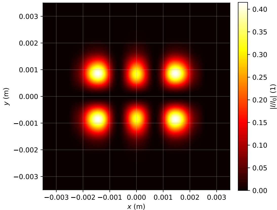
Intensity profile I(x, y, z = 3.105)/I_0 , P_{in}=2.0P_{cr} , artificial time
